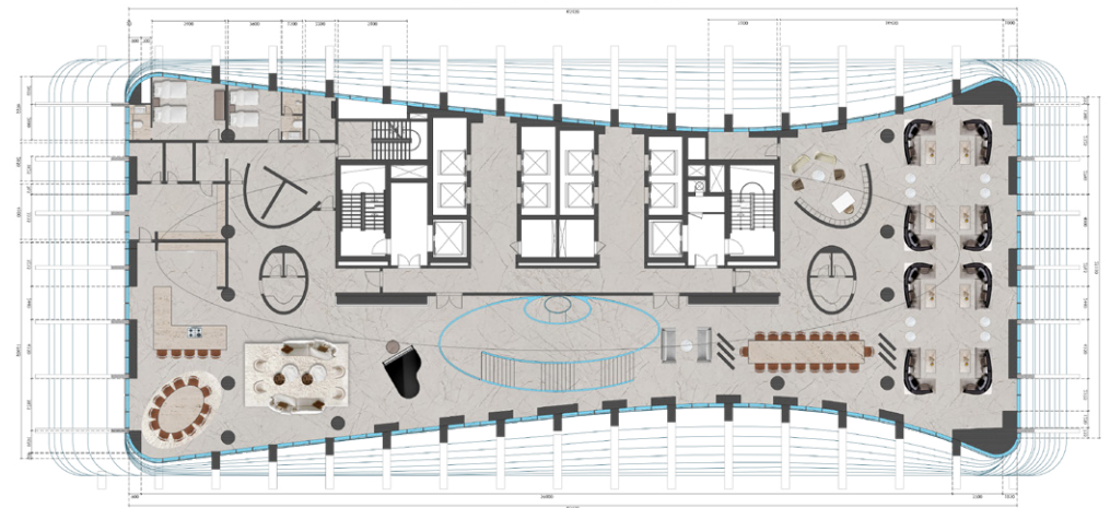
104th Floor Plan LOWER FLOOR PLAN
